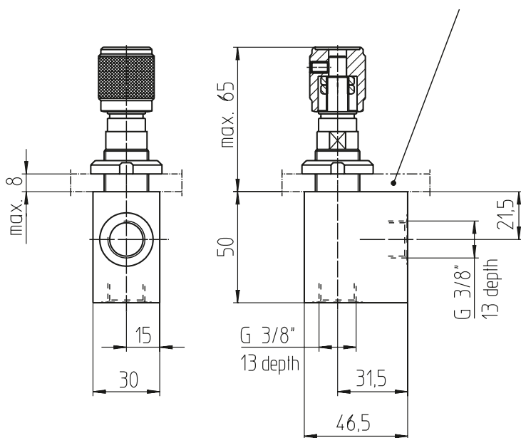
Execution «R» adjustable with knob
